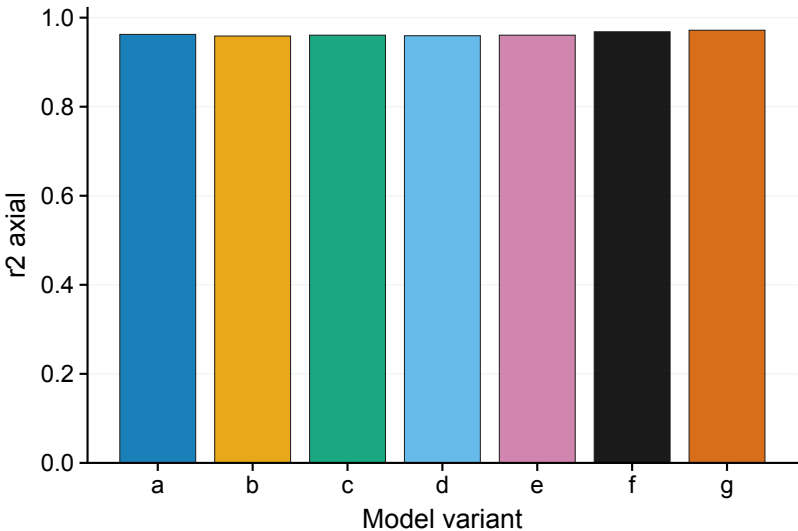
Age Dodge: r2 axial
